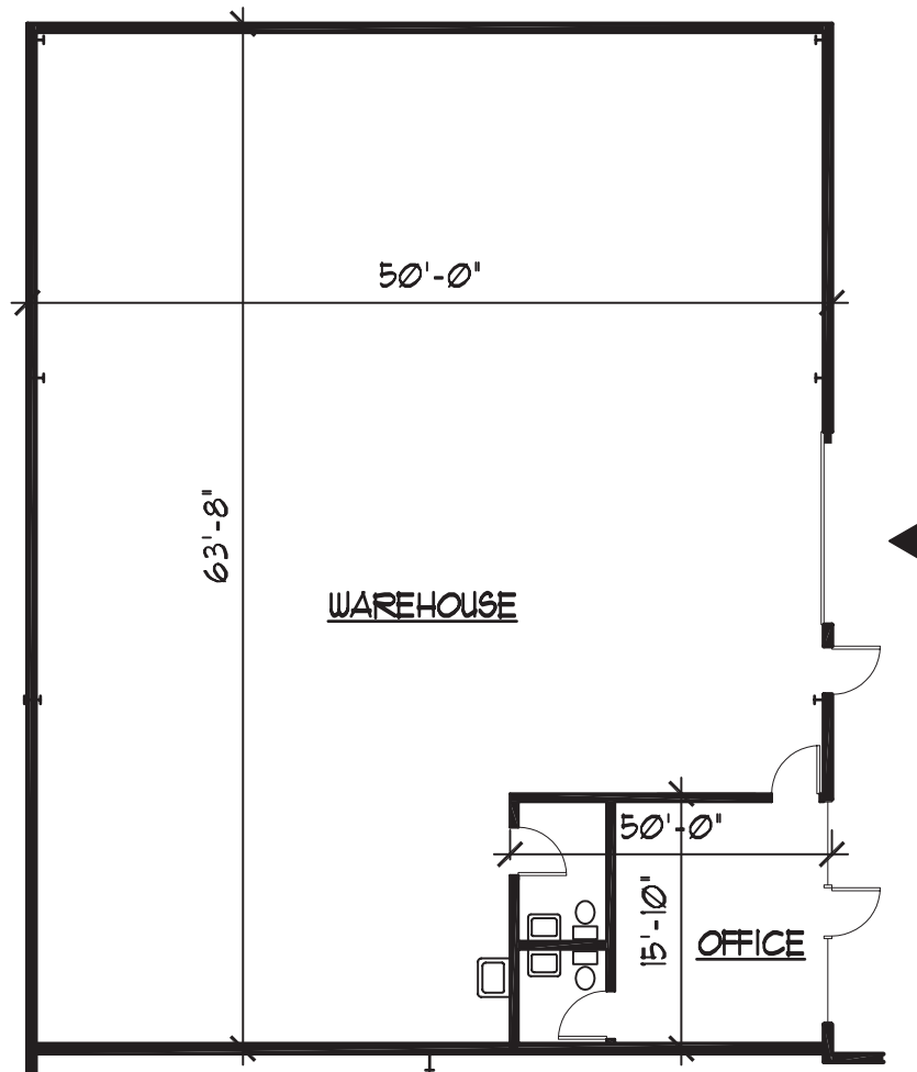
UNIT 5 MAIN FLOOR PLAN
